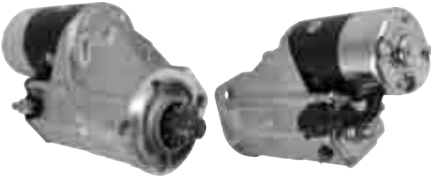
2-2784-ND-2 (Ref# 17311N) Starter - Nippondenso OSGR 2.5kW/12 Volt, CW, 11-Tooth Pinion
