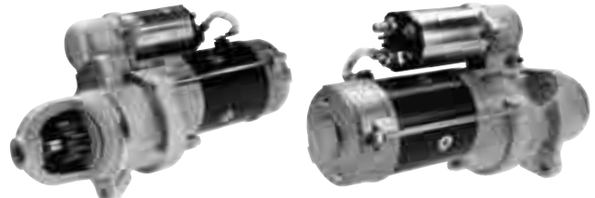
50-8404 (Ref# 6425N) Starter - Delco 28MT Series 12 Volt, CW, 10-Tooth Pinion
